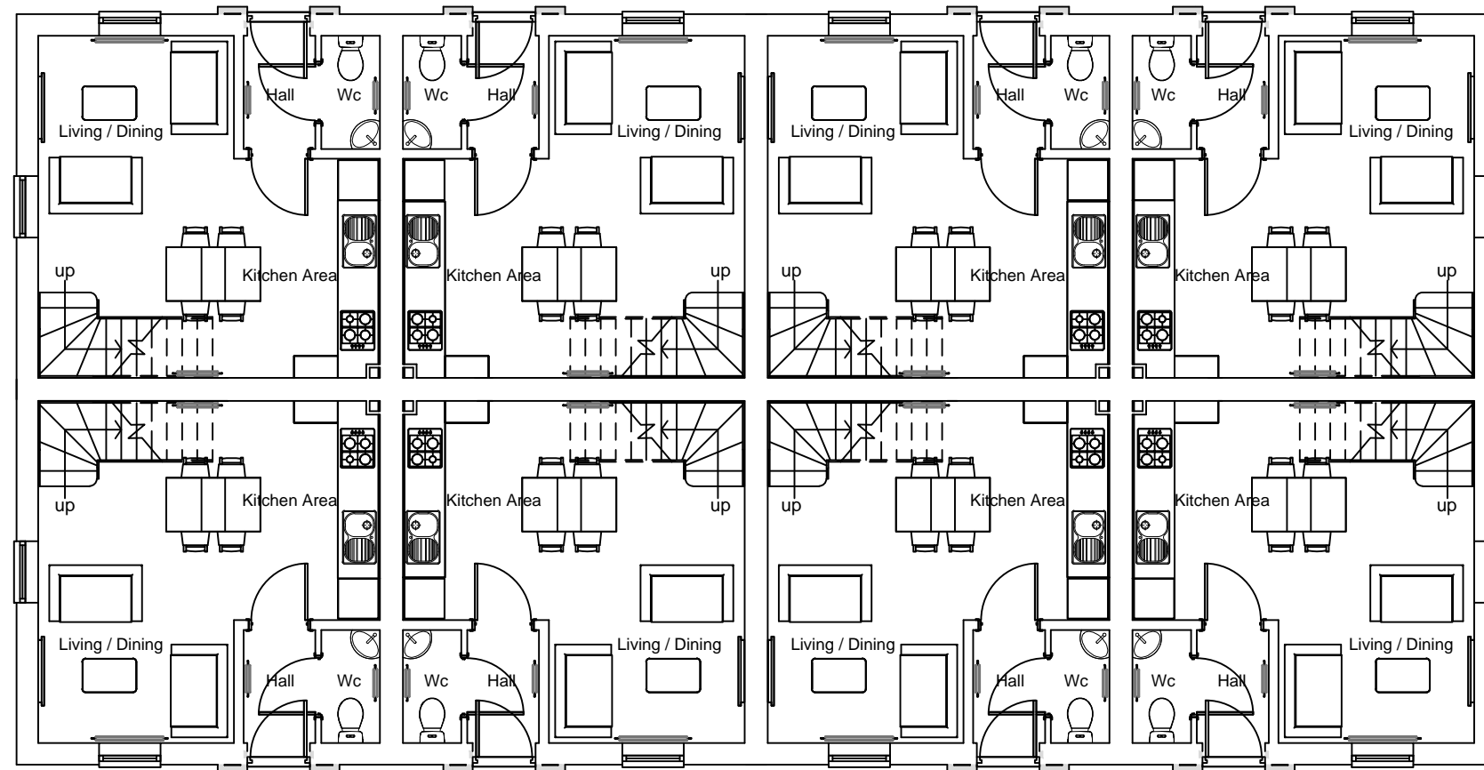
GROUND FLOOR PLAN Type Acomb (end/mid)
